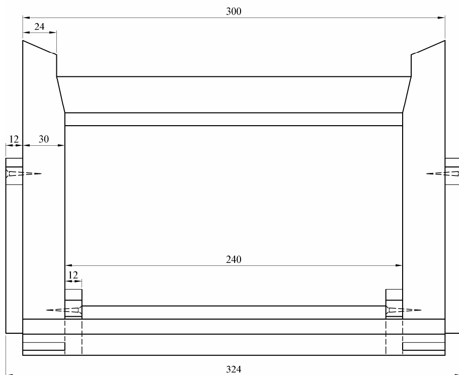
Elevation/Aghaidhchló
